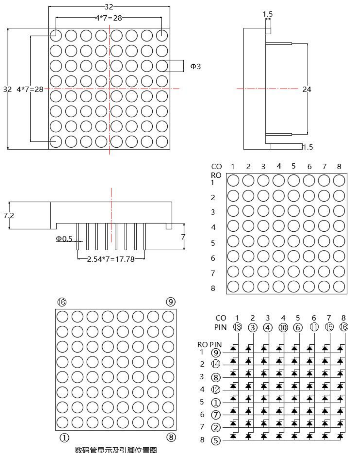
Figure Size & Circuit Principle Diagram : 32mm*32mm*7.2mm
