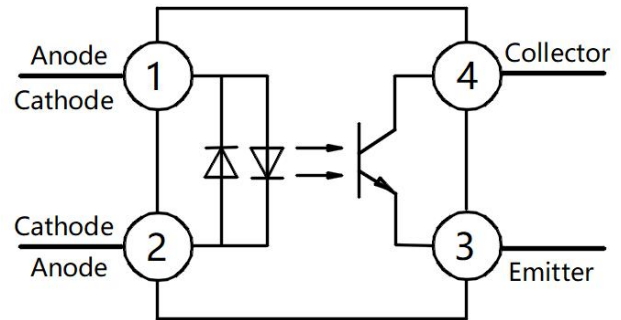
Pin Configuration
