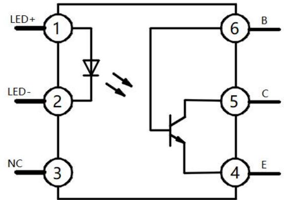
Pin Configuration
