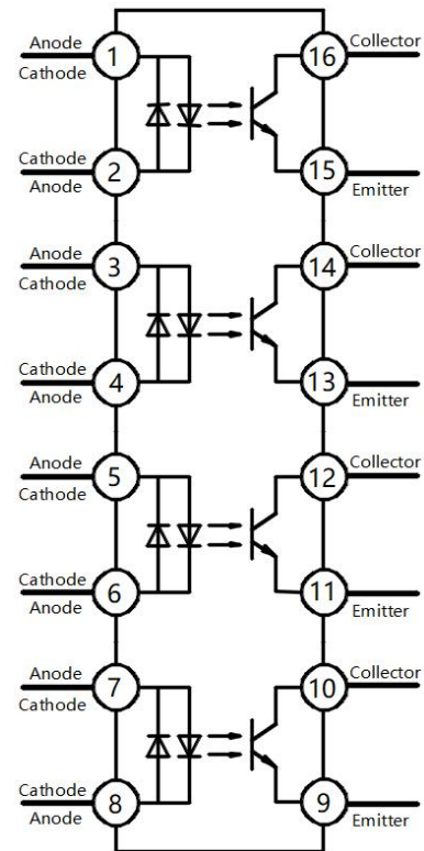
Pin Configuration
