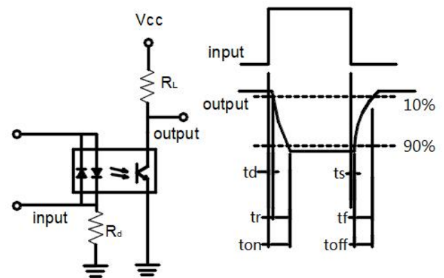
Fig.10 Switching Time Test Circuit & Wave forms
