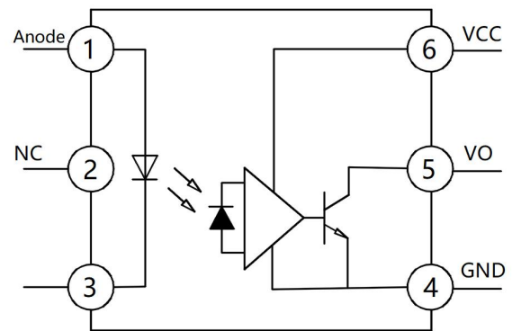
Pin Configuration
