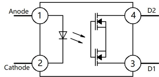
Pin Configuration
