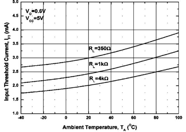
Figure 4. Input Threshold Current vs Ambient Temperature
