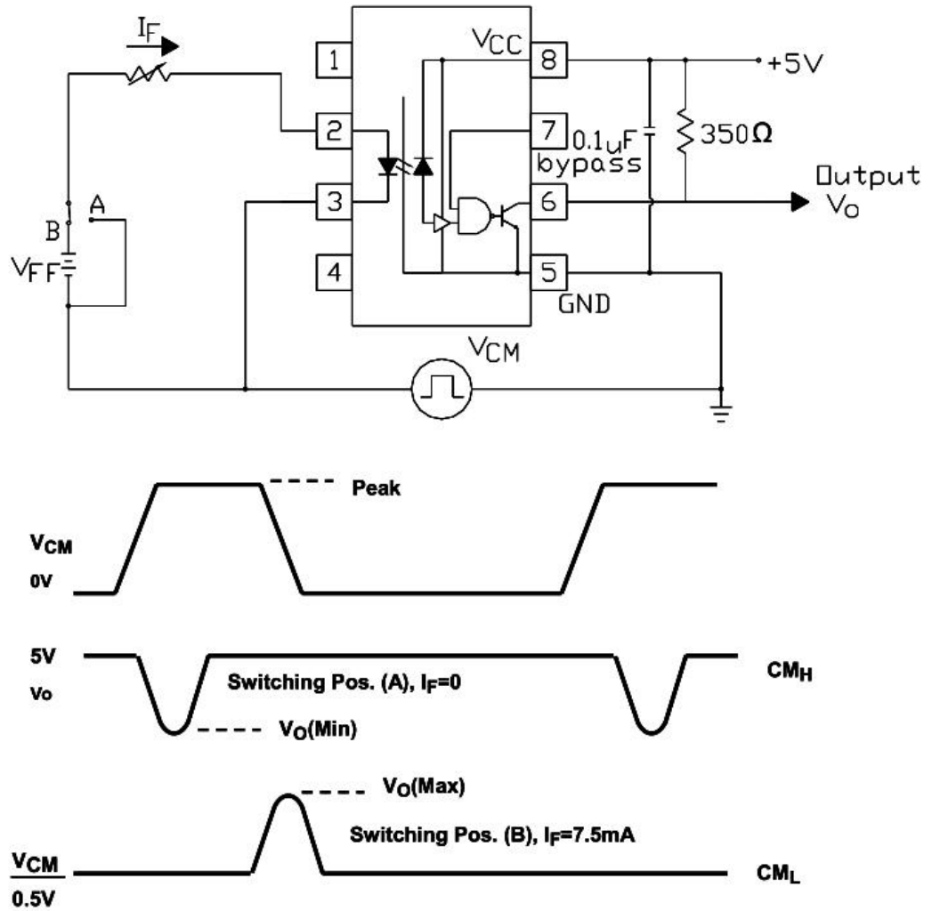
Fig. 14 Test circuit Common mode Transient Immunity
