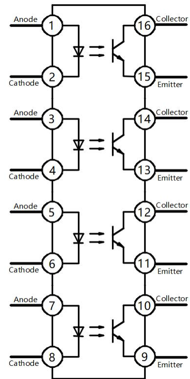
Pin Configuration
