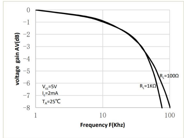
Fig.8 Frequency Response
