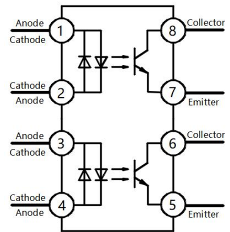
Pin Configuration
