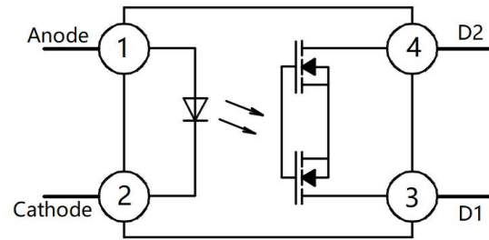
Pin Configuration
