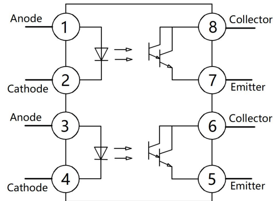
Pin Configuration
