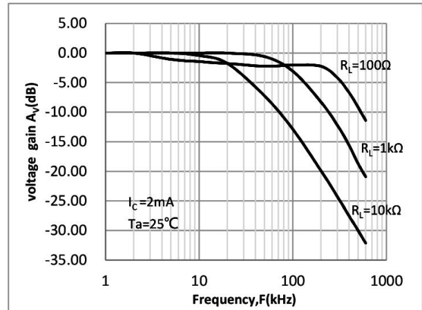
Fig.8 Frequency Response
