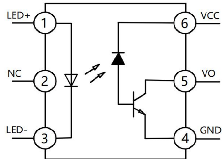
Pin Configuration
