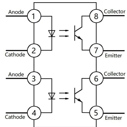
Pin Configuration
