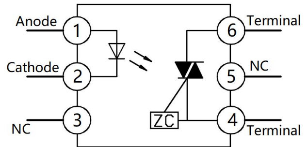
Pin Configuration
