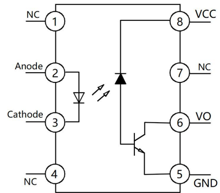
Pin Configuration
