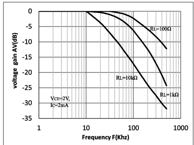
Fig.10 Frequency Response
