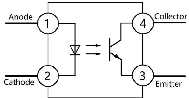
Pin Configuration
