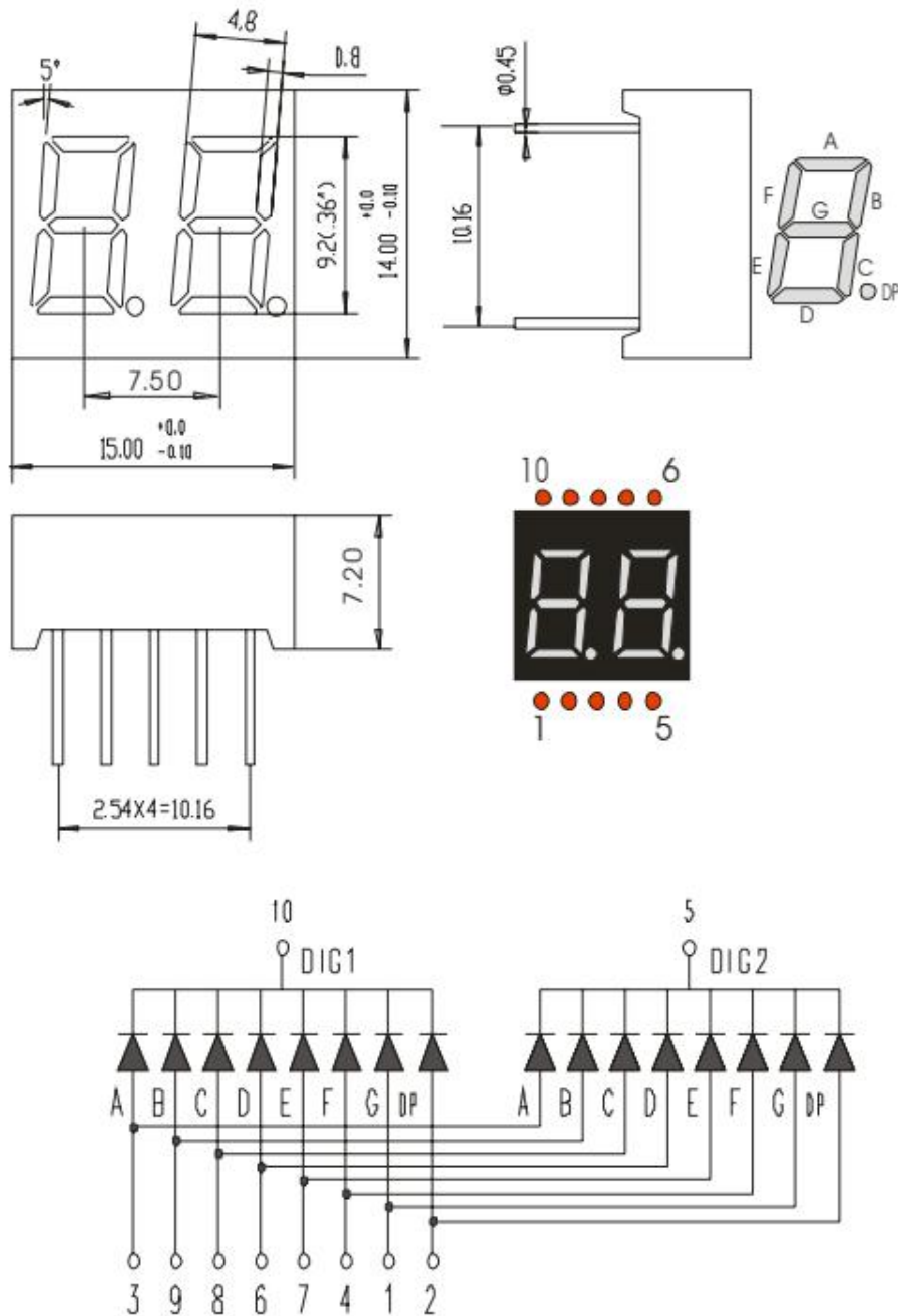
Figure Size & Circuit Principle Diagram : 15mm×14mm×7.2mm
