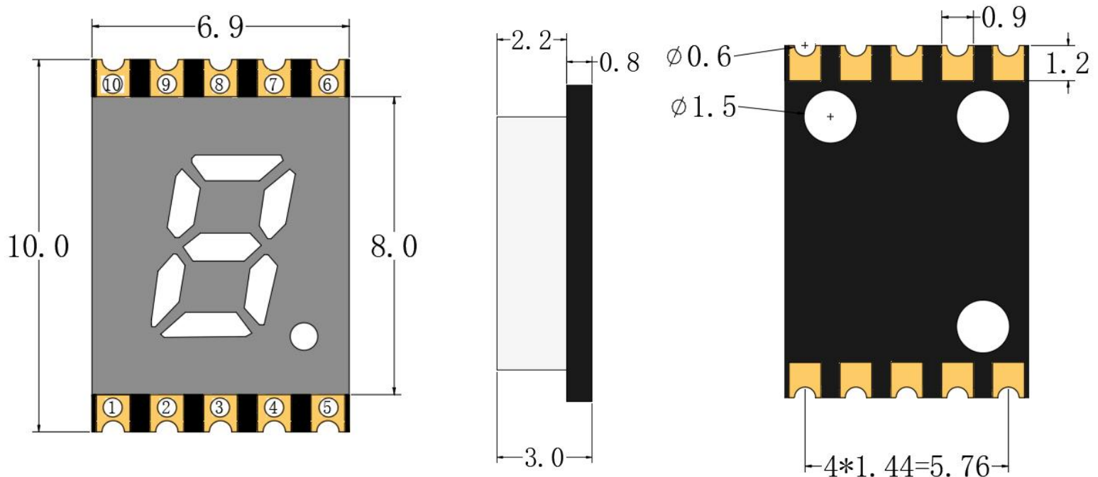
Figure Size & Circuit Principle Diagram : 10mm×6.9mm×3.0mm
