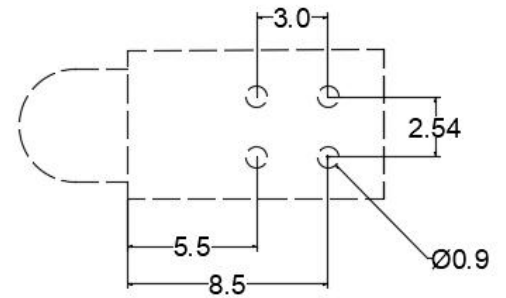
建议焊盘尺寸 Recommended Soldering Pattern
