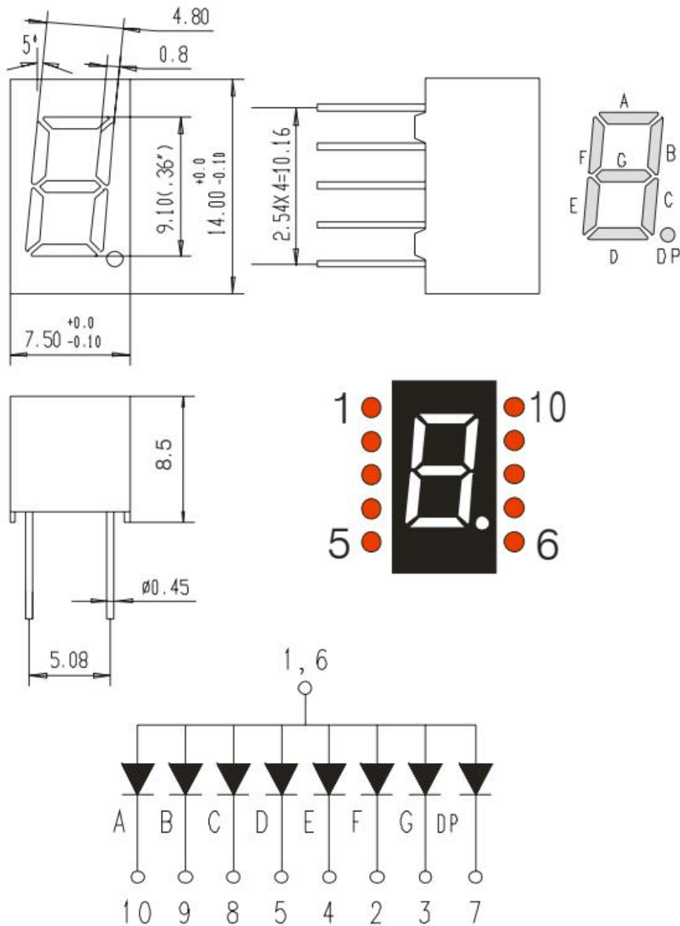
Figure Size & Circuit Principle Diagram : 7.5mm×14mm×8.5mm
