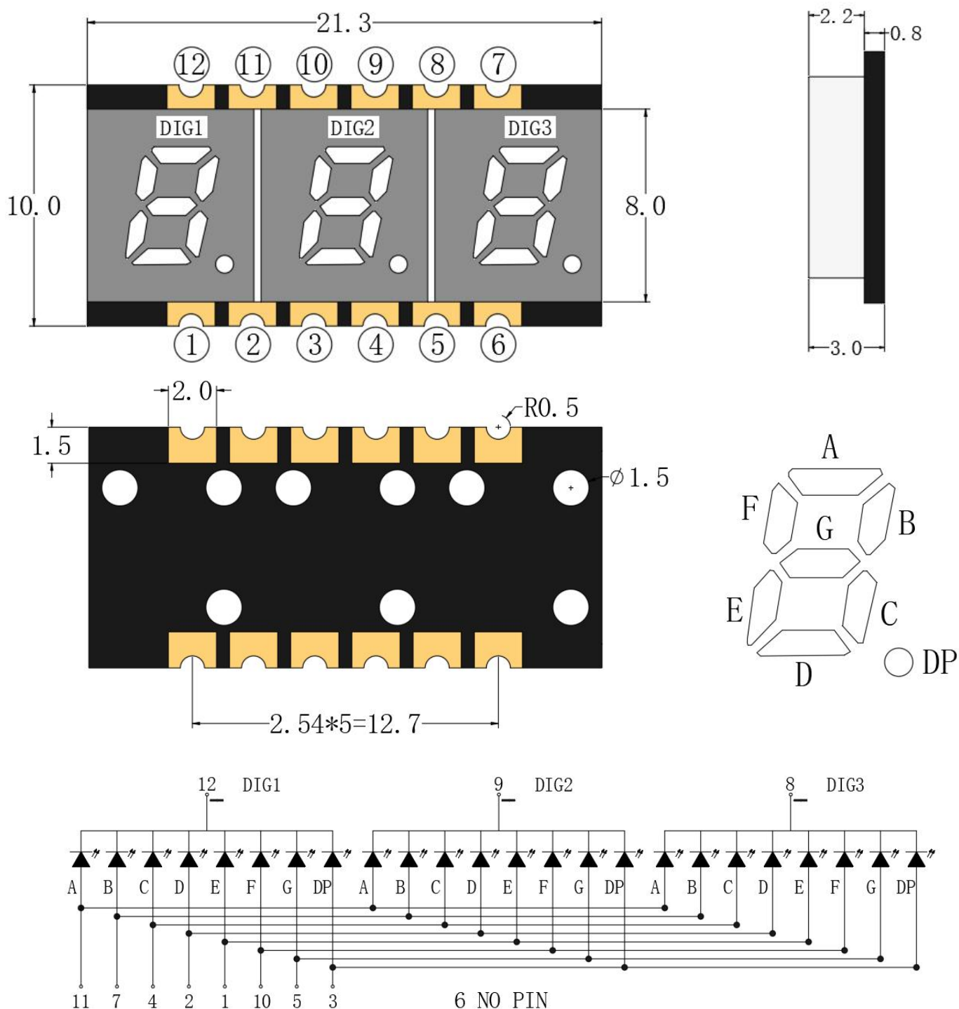
Figure Size & Circuit Principle Diagram : 21.3mm×10mm×3.0mm
