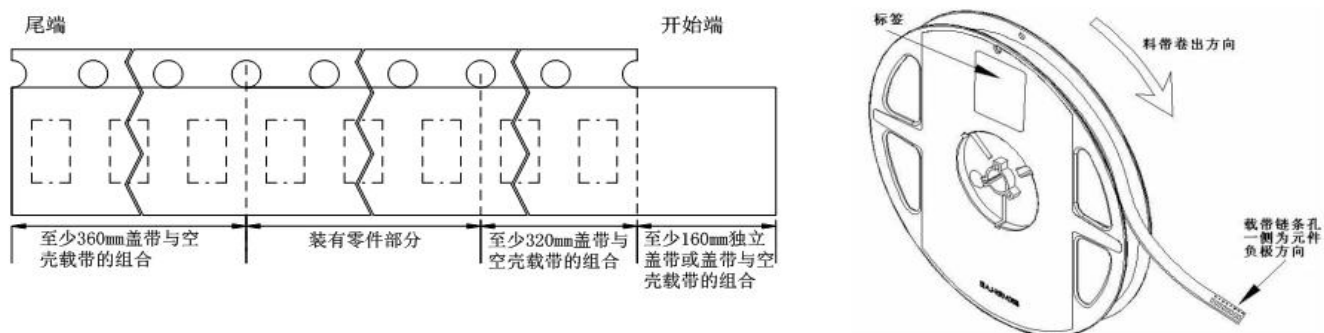
◇ 圆盘及载带卷出方向及空穴规格 Disk and carrier belt direction of roll and hole dimensions
