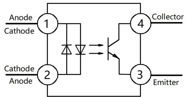
Pin Configuration
