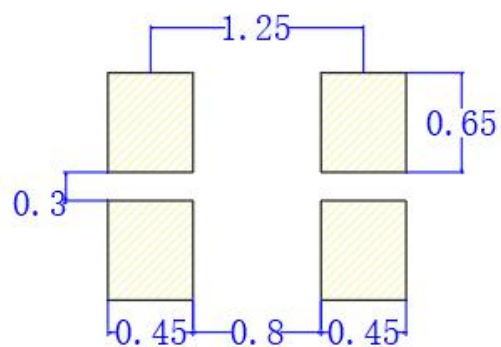
建议焊盘尺寸 Recommended Soldering Pattern
