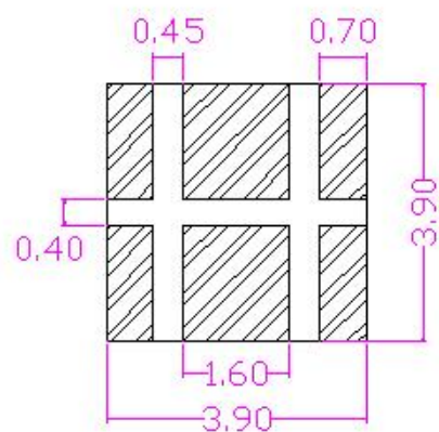
建议焊盘尺寸: Recommended Soldering Pattern
