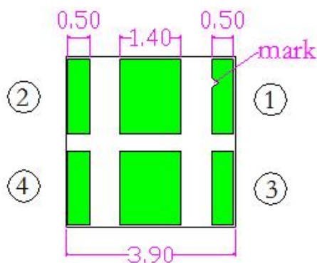
建议焊盘尺寸: Recommended Soldering Pattern
