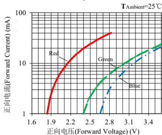
伏安特性 Volt-Ampere Characteristics
