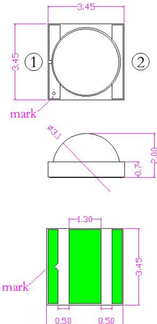
建议焊盘尺寸: Recommended Soldering Pattern
