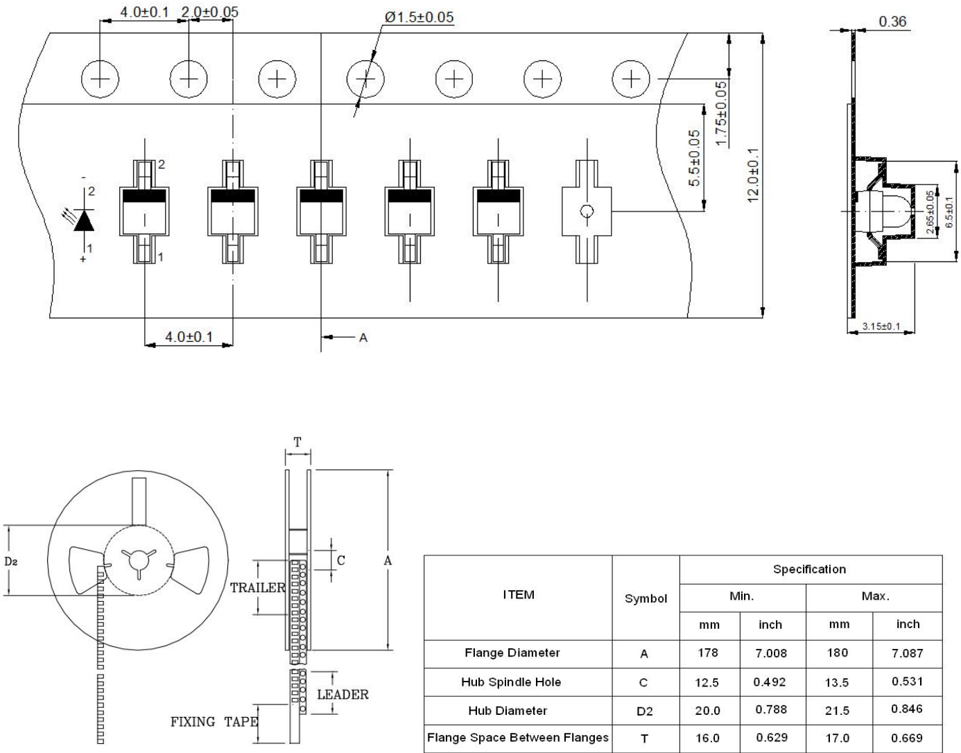
载带与圆盘尺寸 Belt and disk dimensions
