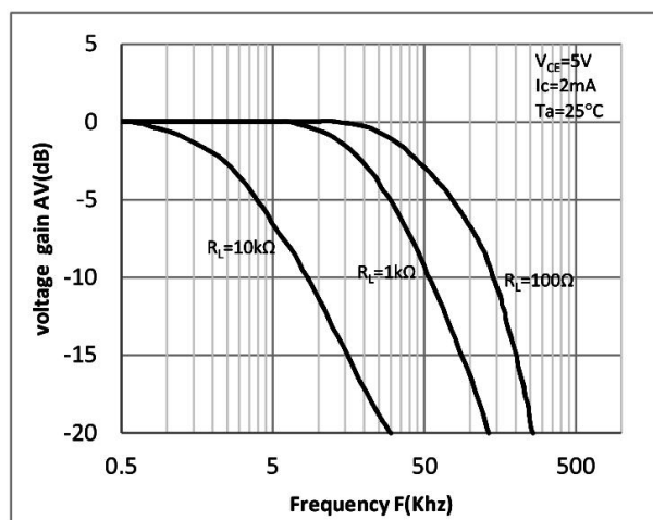
Fig.8 Frequency Response
