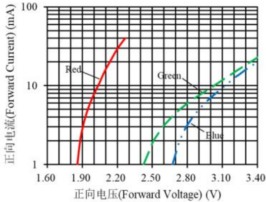
伏安特性 Volt-Ampere Characteristics T_{Ambient}=25^{\circ}C
