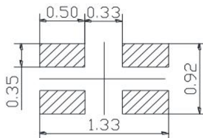
建议焊盘尺寸: Recommended Soldering Pattern
