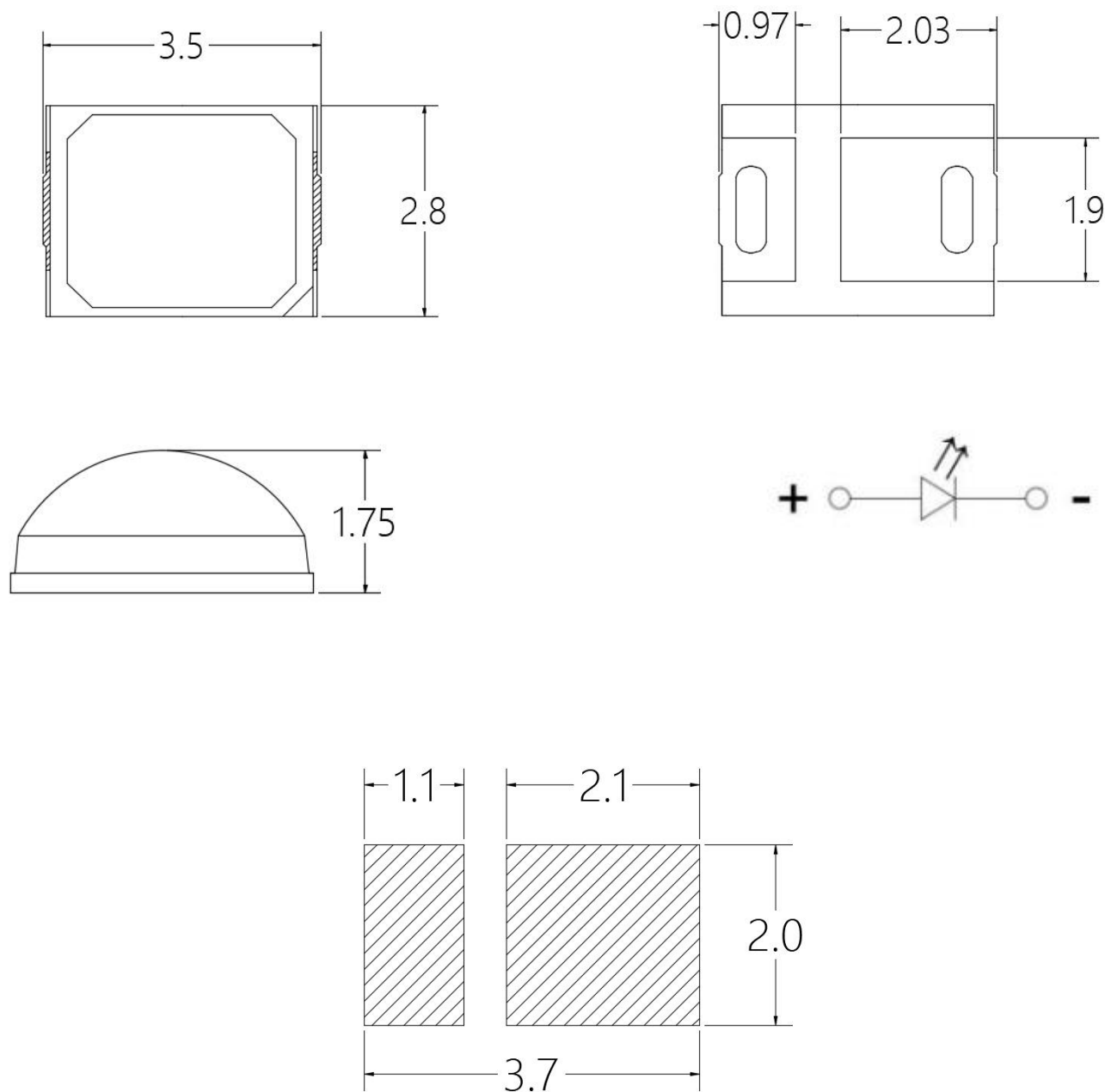
建议焊盘尺寸 Recommended Soldering Pattern
