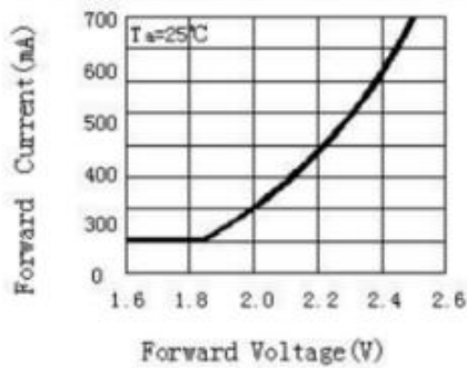
电压与电流关系, 温度=25℃ Forward Voltage VS Forward Current, Ta=25℃
