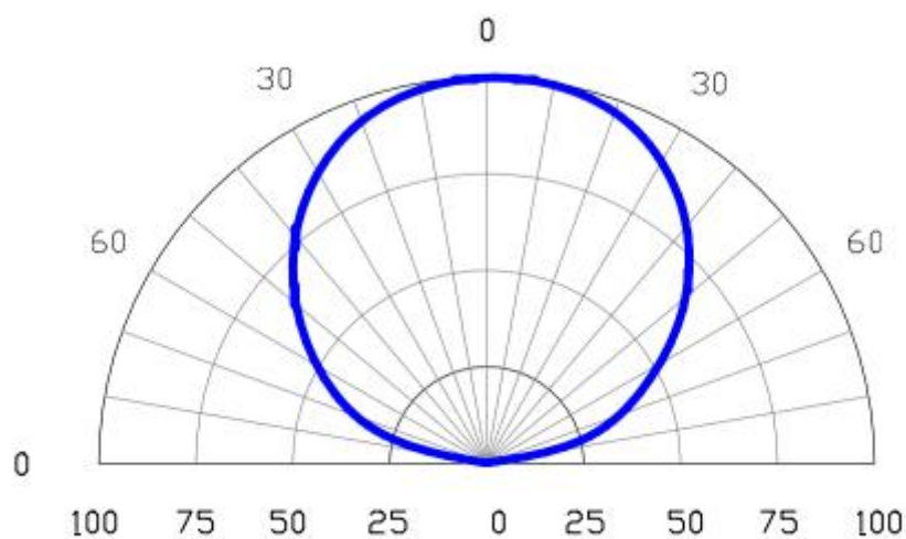
Beam Patter
