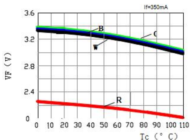
Temperature vs Forward Voltage
