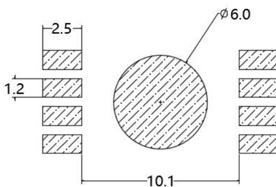
建议焊盘尺寸 Recommended Soldering Pattern
