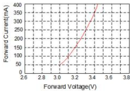
Forward current - voltage curve
