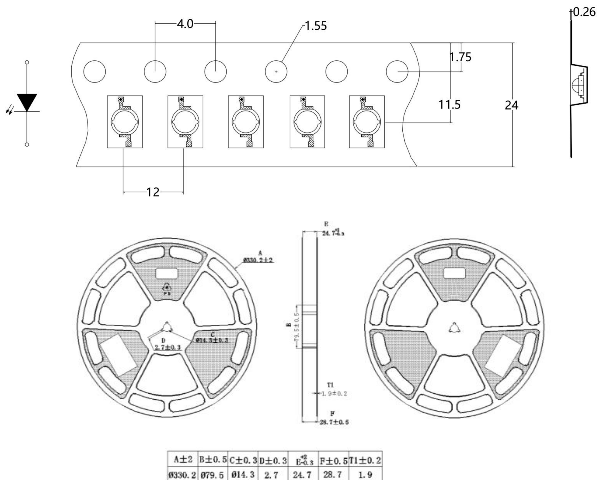
载带与圆盘尺寸 Belt and disk dimensions
