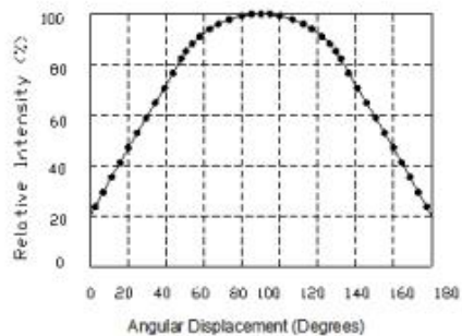
LED光强分布曲线(1000mA测试) Intensity distribution curve (1000mA test):
