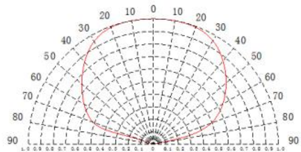
LED光强分布曲线(1000mA测试) Intensity distribution curve (1000mA test):
