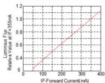
Forward current - luminous intensity curve
