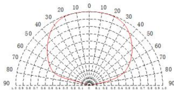
LED光强分布曲线(1000mA测试) Intensity distribution curve (1000mA test):
