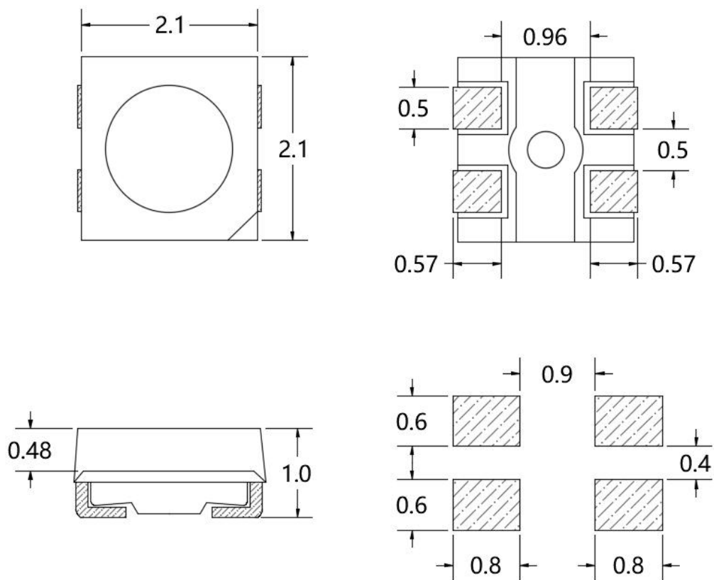
建议焊盘尺寸 Recommended Soldering Pattern
