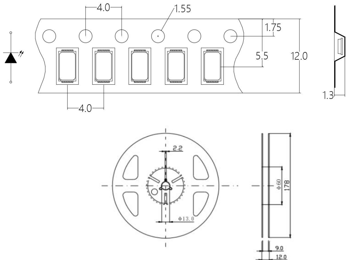
载带与圆盘尺寸 Belt and disk dimensions
