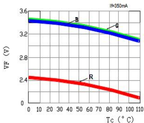
Temperature vs Forward Voltage
