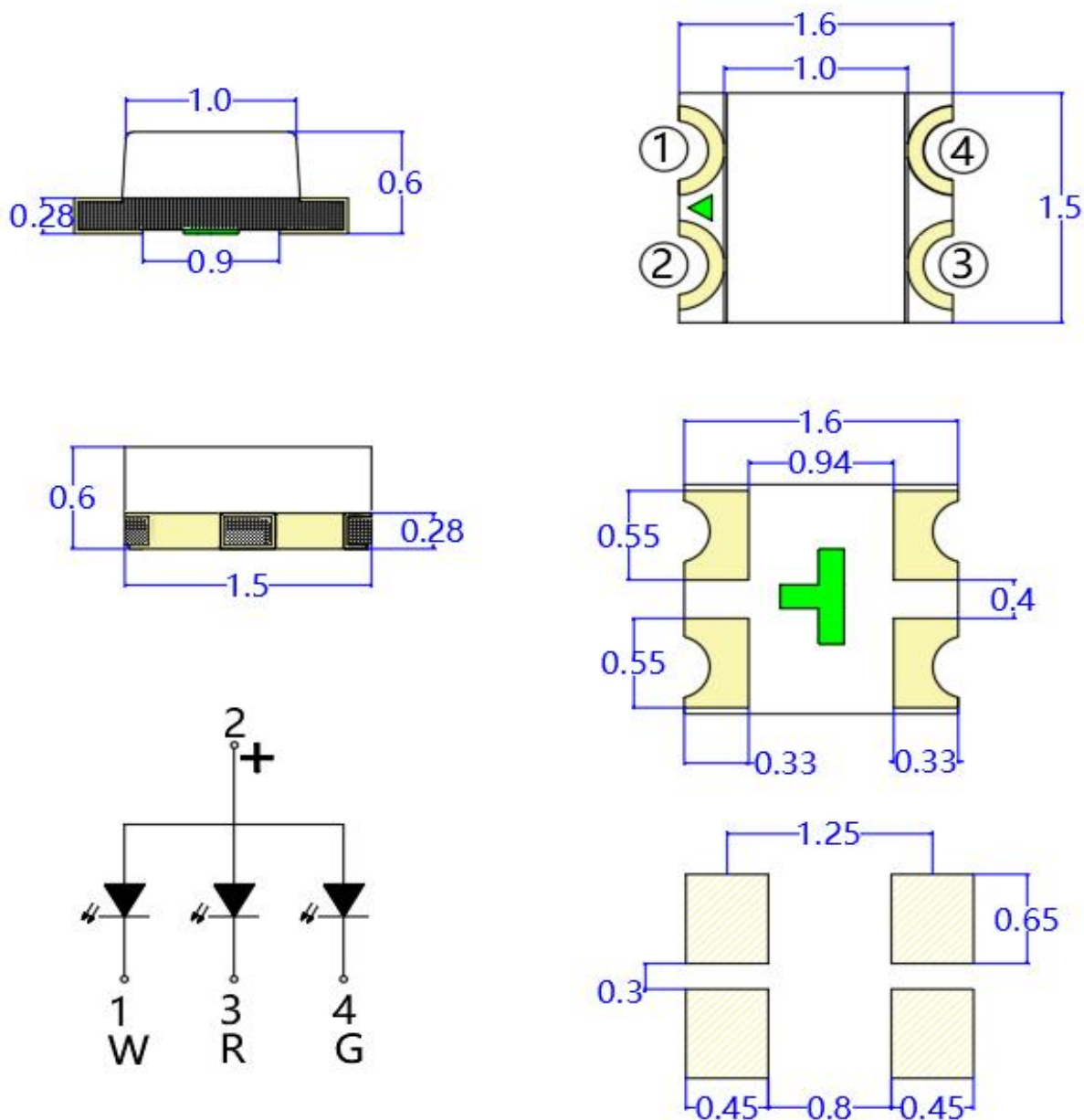
建议焊盘尺寸 Recommended Soldering Pattern
