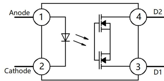
Pin Configuration
