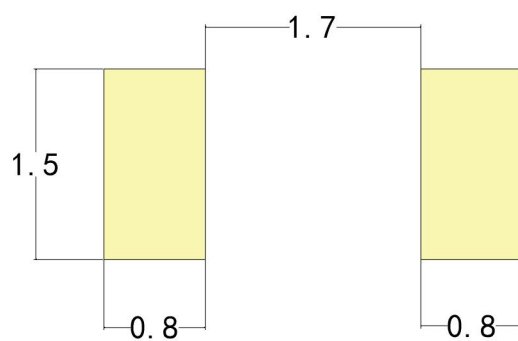
建议焊盘尺寸 Recommended Soldering Pattern
