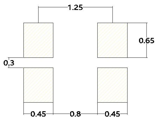
建议焊盘尺寸 Recommended Soldering Pattern
