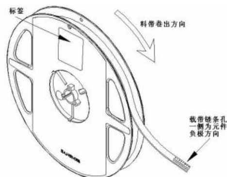
◆ 圆盘及载带卷出方向及空穴规格 Disk and carrier belt direction of roll and hole dimensions
