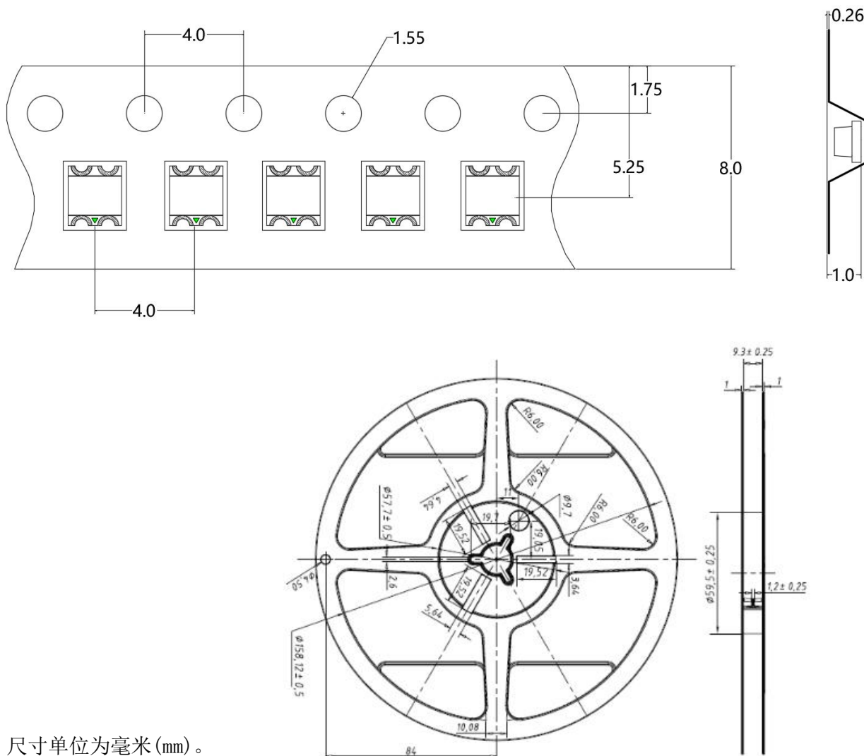
载带与圆盘尺寸 Belt and disk dimensions
