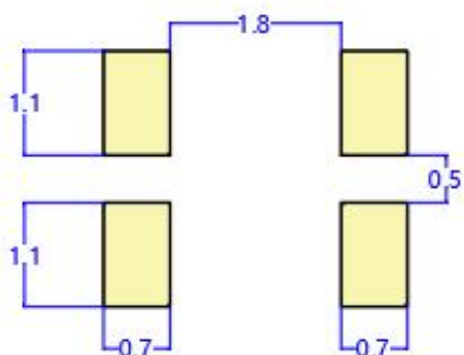
建议焊盘尺寸 Recommended Soldering Pattern
