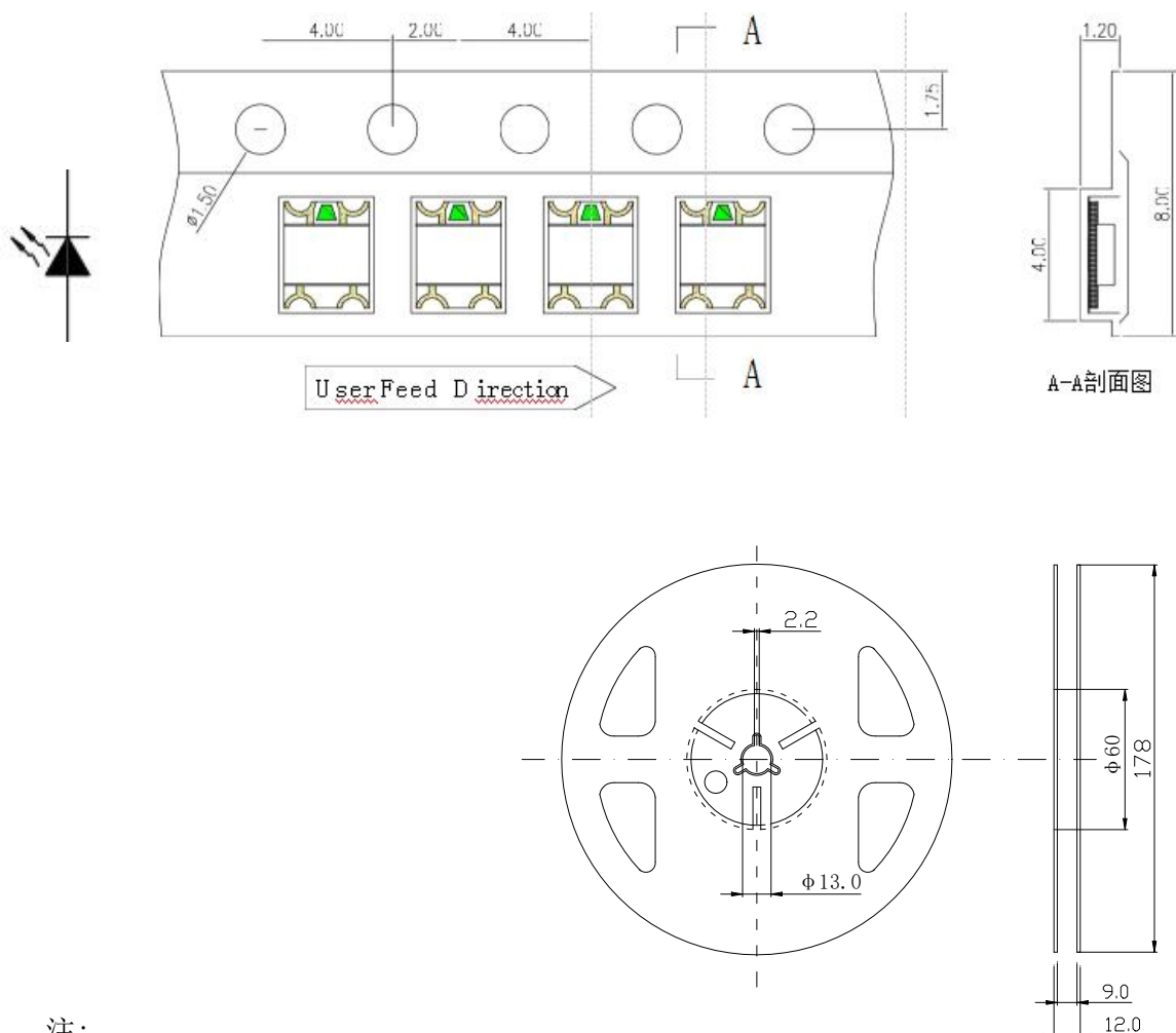
载带与圆盘尺寸 Belt and disk dimensions
