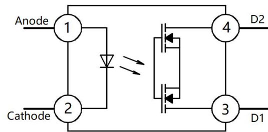
Pin Configuration
