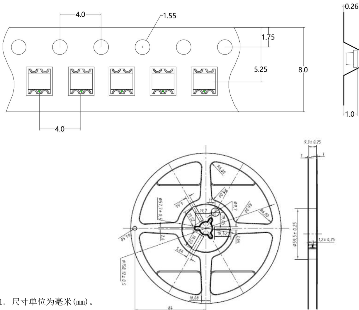
载带与圆盘尺寸 Belt and disk dimensions
