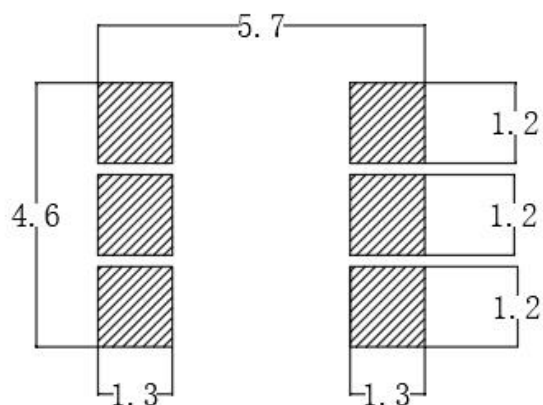
建议焊盘尺寸 Recommended Soldering Pattern
