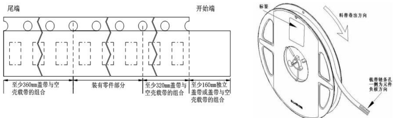
◆ 圆盘及载带卷出方向及空穴规格 Disk and carrier belt direction of roll and hole dimensions
