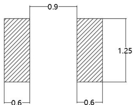
建议焊盘尺寸 Recommended Soldering Pattern
